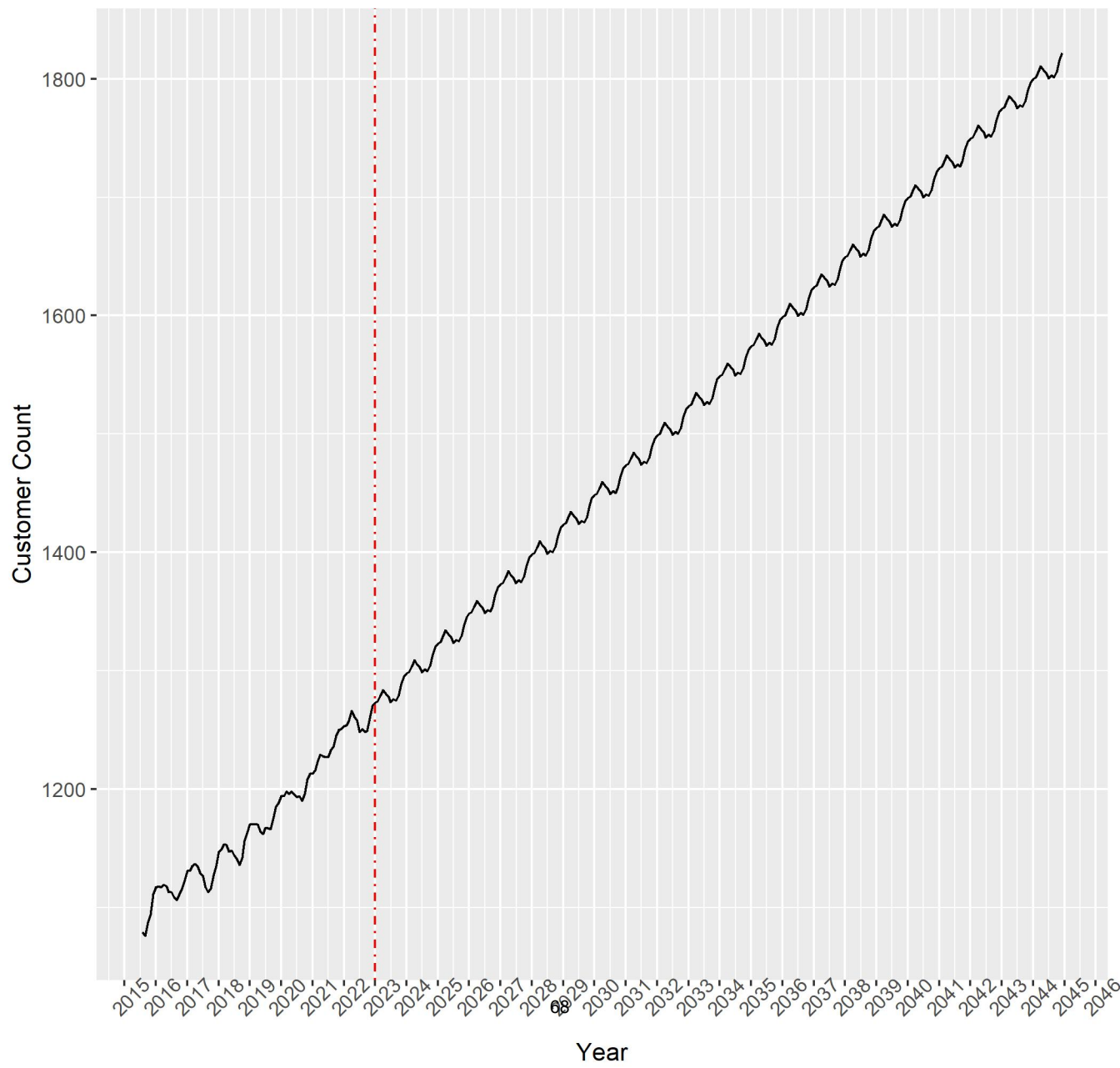
Fremont.res: Dynamic Linear Regression Model: ARIMA Only
