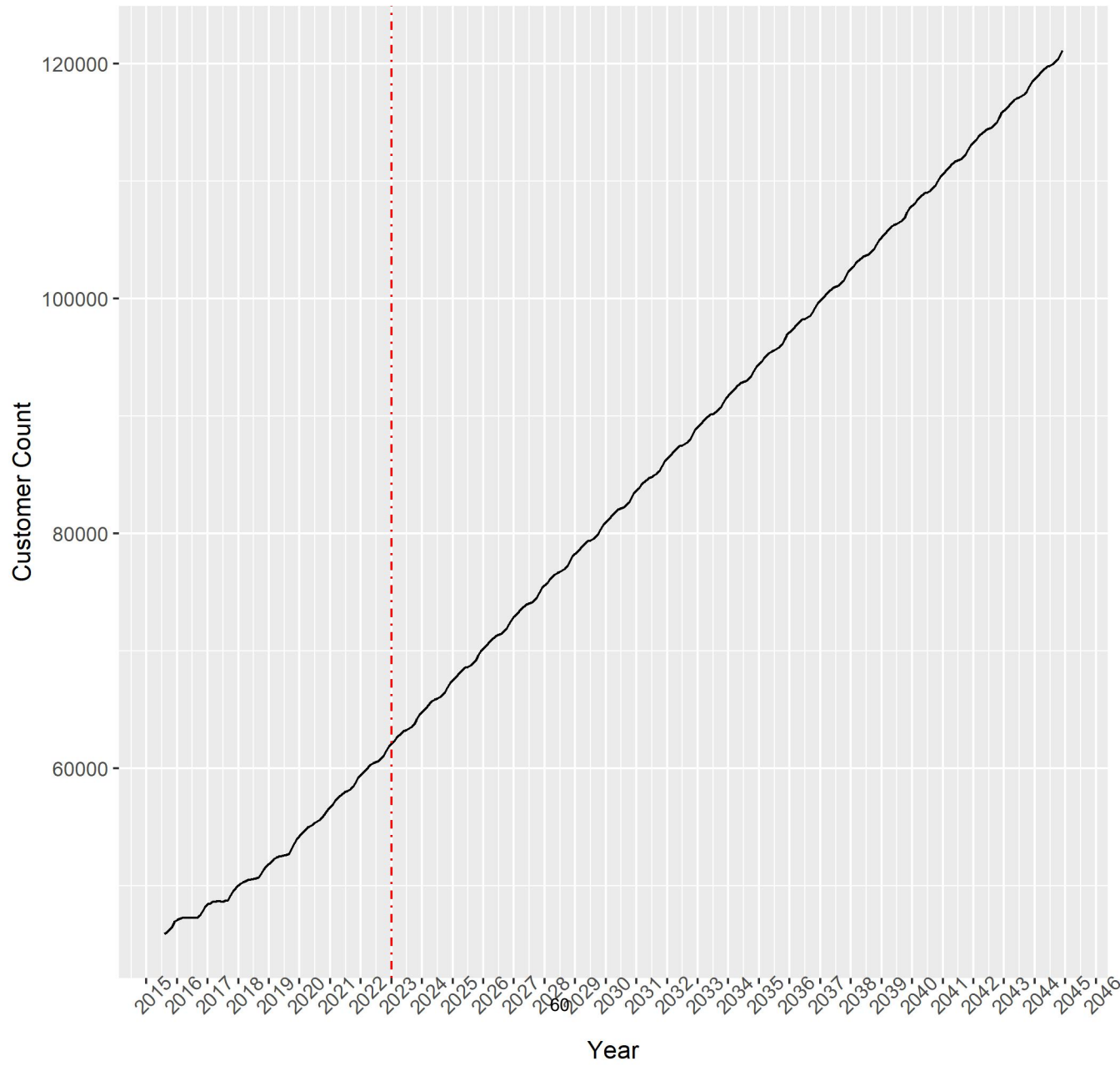
Canyon.res: Dynamic Linear Regression Model: ARIMA Only
