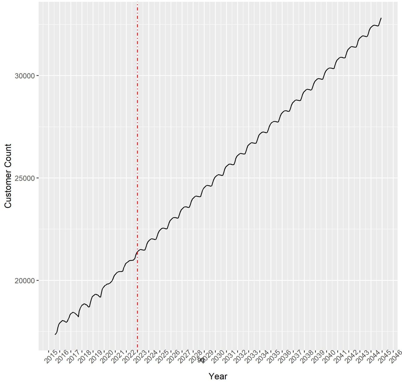
Twin.Falls.res: Dynamic Linear Regression Model: ARIMA Only
