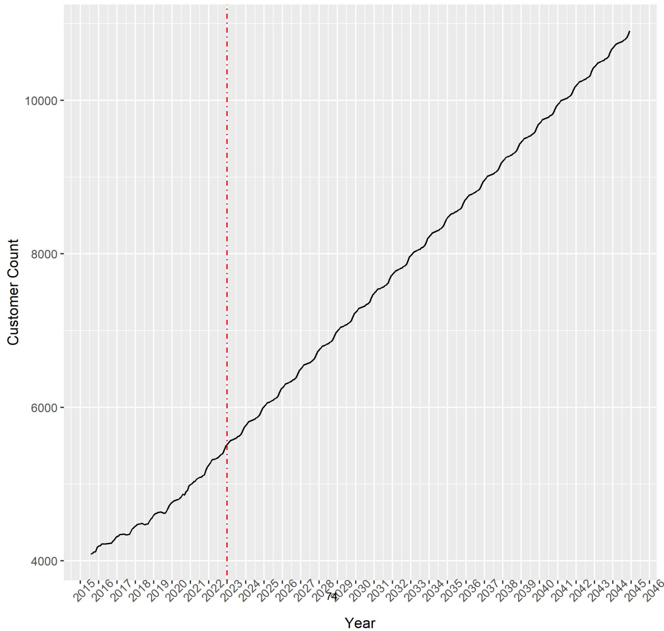
Jefferson.res: Dynamic Linear Regression Model: ARIMA Only
