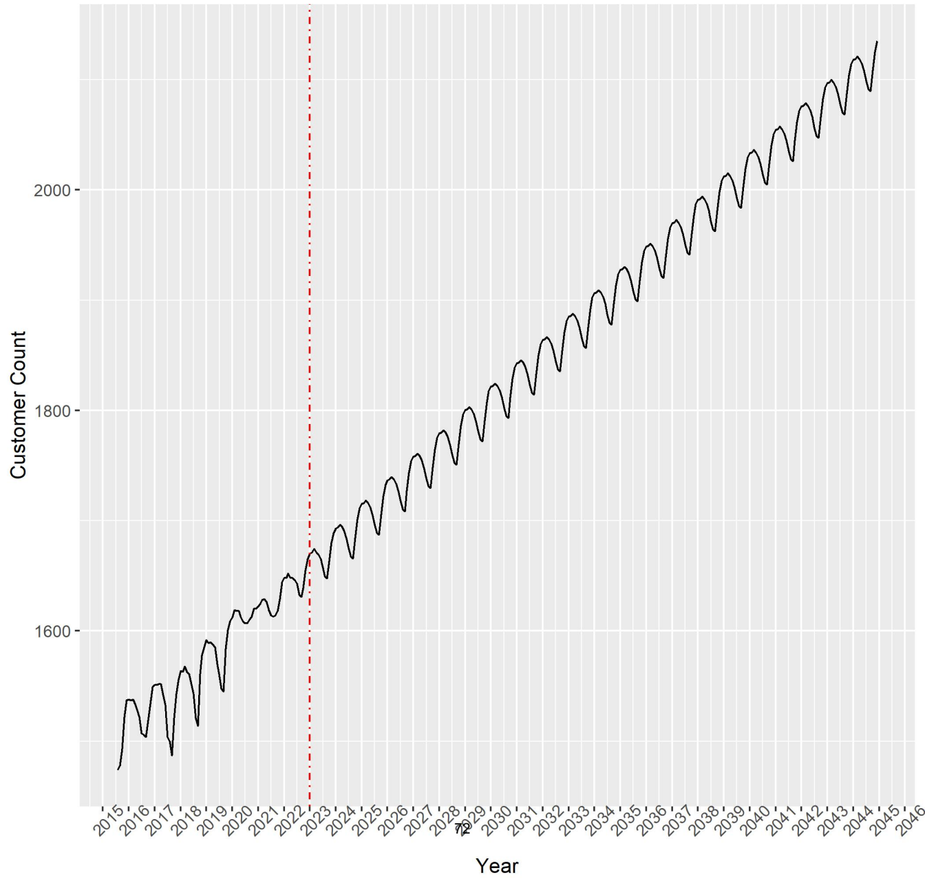
Gooding.res: Dynamic Linear Regression Model: ARIMA Only
