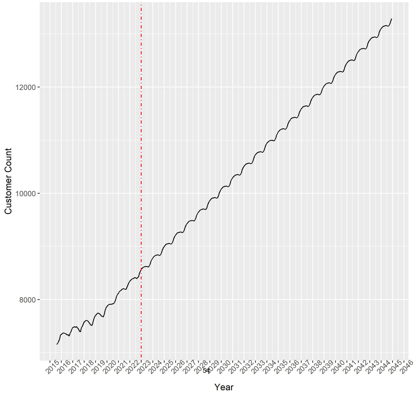
Bingham.res: Dynamic Linear Regression Model: ARIMA Only
