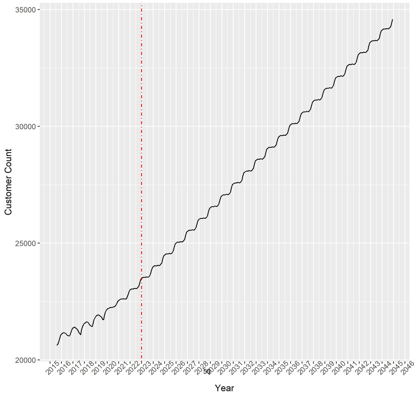
Bannock.res: Dynamic Linear Regression Model: ARIMA Only
